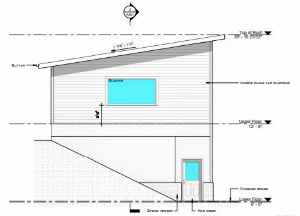
④ West 1/4" = 1'-0"
