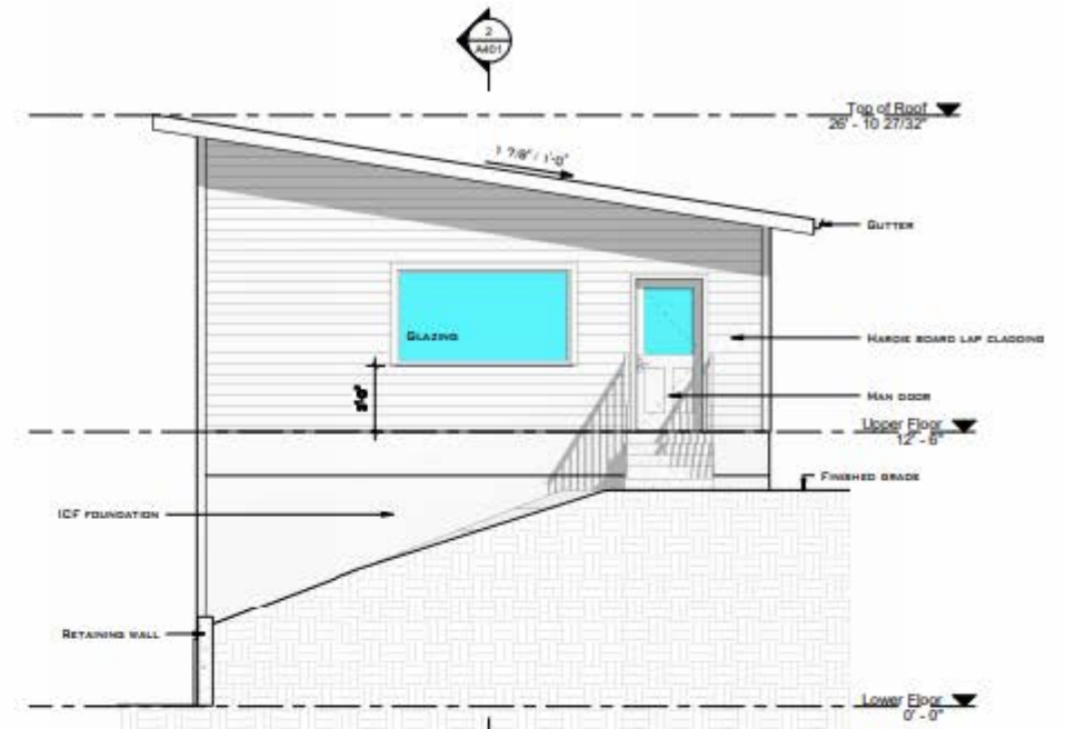
② East 1/4" = 1'-0"
