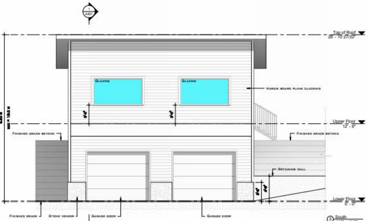
③ South 1/4" = 1'-0"
