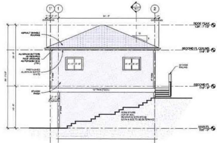
③ SOUTH 1/4" = 1'-0"
