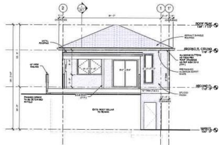
③ SOUTH 1/4" = 1'-0"
