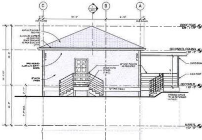
① WEST 1/4" = 1'-0"
