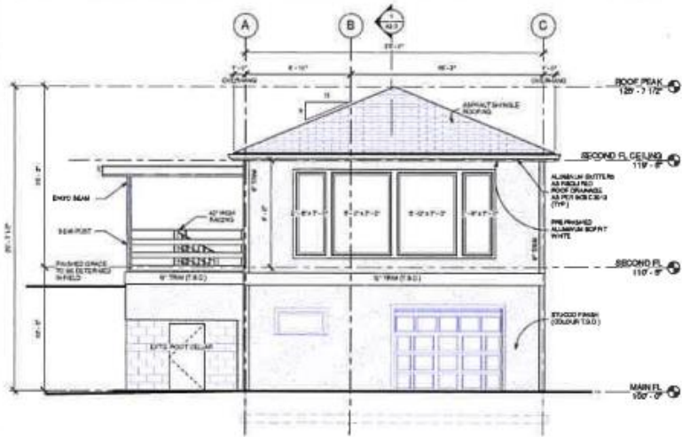
① WEST 1/4" = 1'-0"
