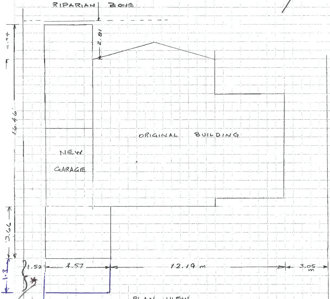
PLAN VIEW 4257 MILL RD
