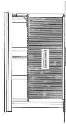
SOUTH ELEVATION SCALE 1/4" = 1'-0"
